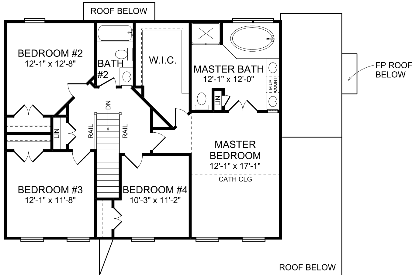
SECOND FLOOR PLAN THE POTOMAC II
