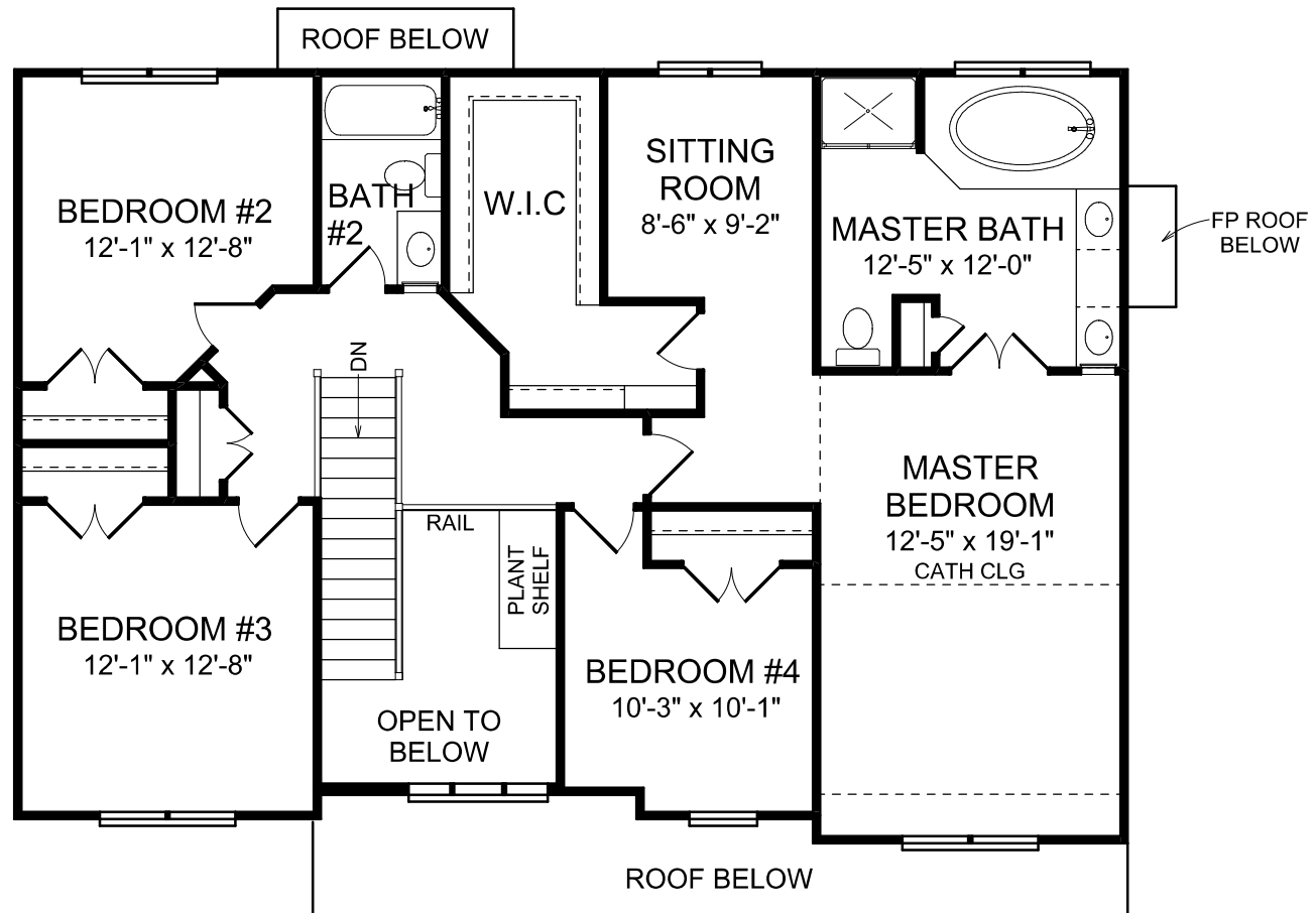
SECOND FLOOR PLAN THE CYPRESS SPRING
