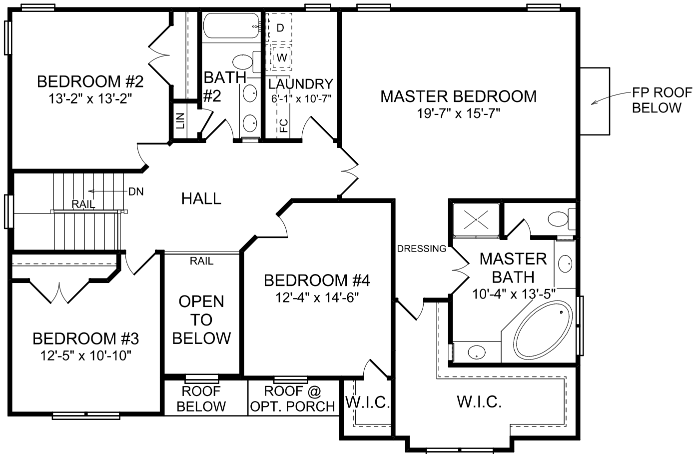
SECOND FLOOR PLAN THE CHELSEA II
