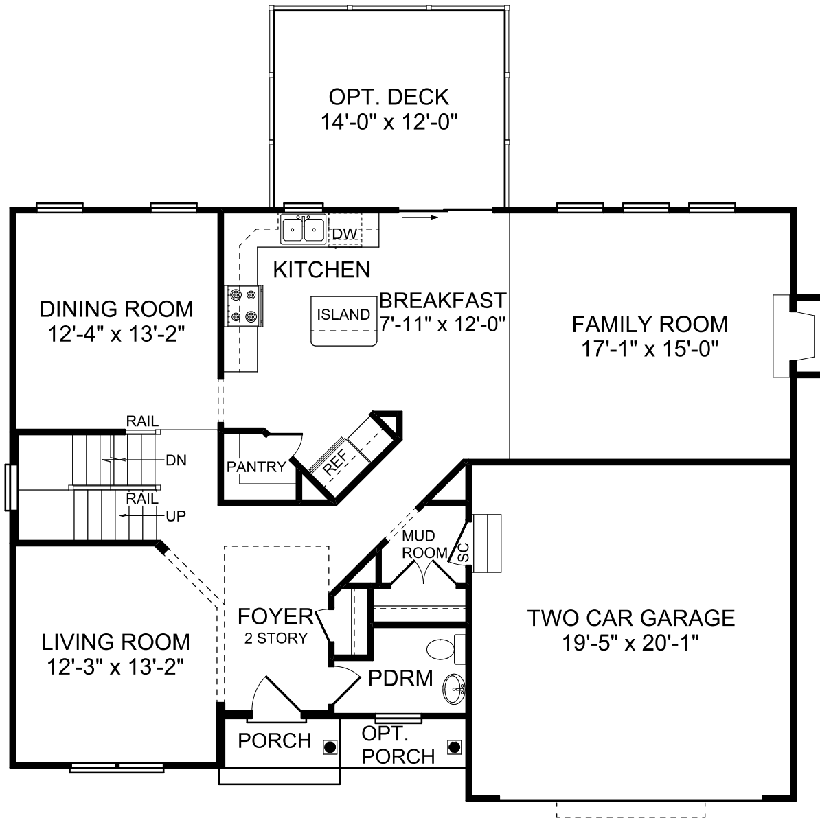
FIRST FLOOR PLAN THE CHELSEA II
