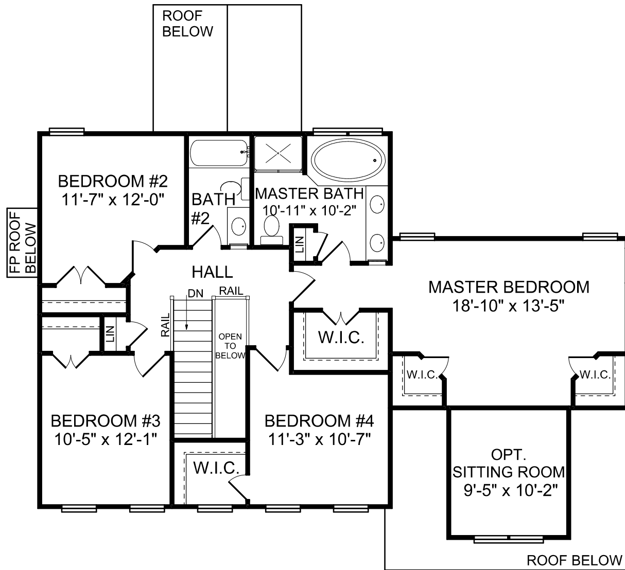
SECOND FLOOR PLAN THE ST. JAMES II
