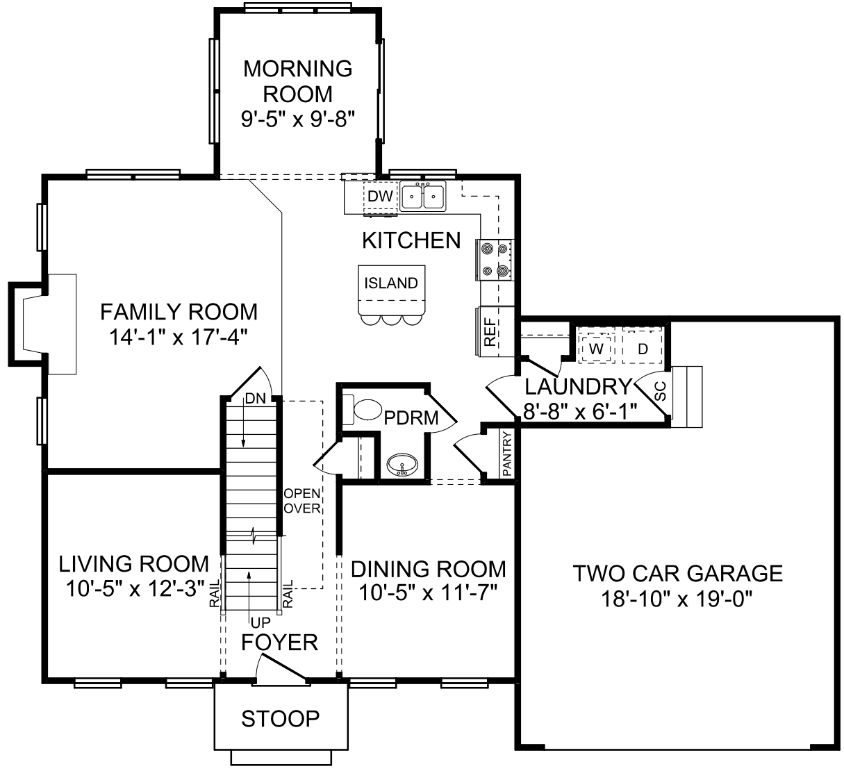
FIRST FLOOR PLAN THE ST. JAMES II
